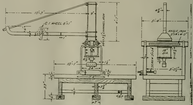
STRAIGHTENING TABLE, DELAWARE & HUDSON CO.
